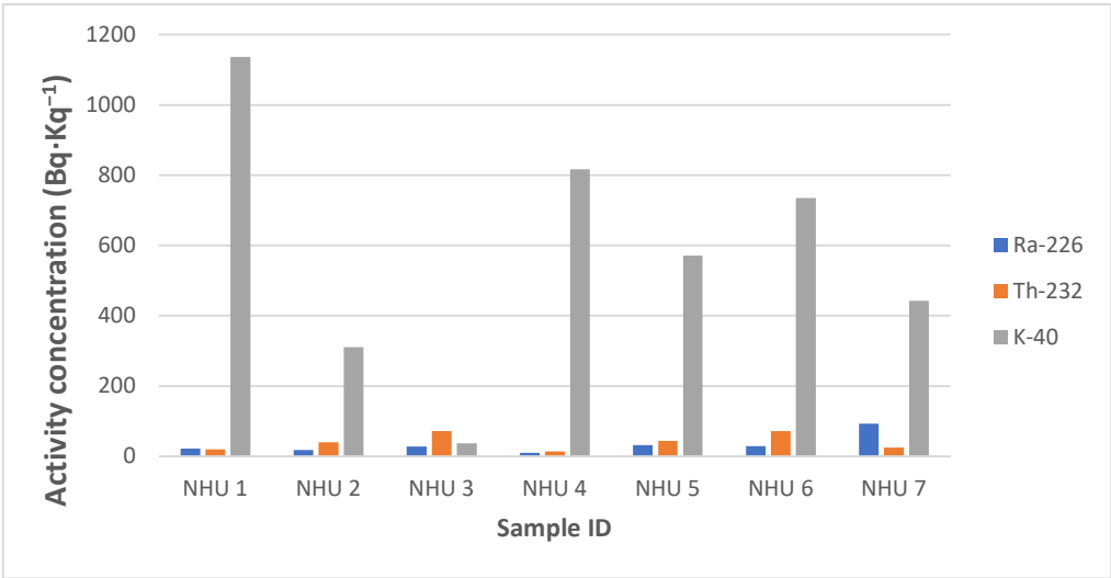
Fig. 4. Activity concentrations of ^{226}\text{Ra} , ^{232}\text{Th} , and ^{40}\text{K} for rock samples collected from Nahuta.
