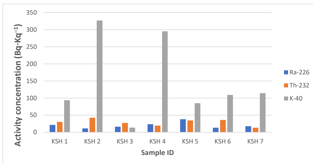
Fig. 6. Activity concentrations of ^{226}\text{Ra} , ^{232}\text{Th} , and ^{40}\text{K} for rock samples collected from Kashere.
