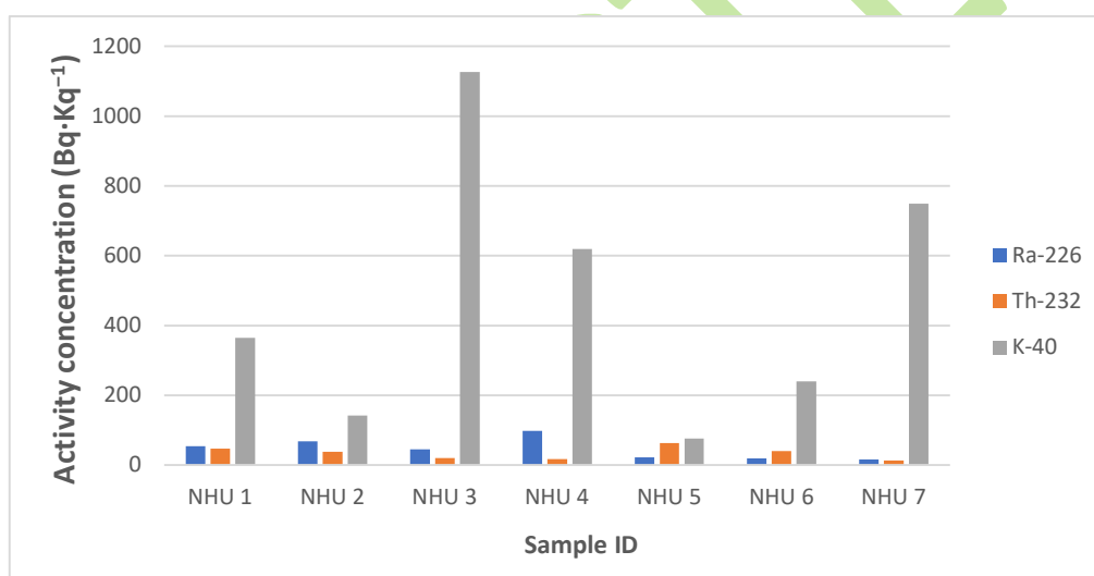
Fig. 3. Activity concentrations of ^{226}\text{Ra} , ^{232}\text{Th} , and ^{40}\text{K} for soil samples collected from Nahuta.
