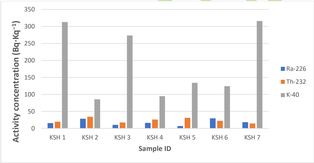
Fig. 5. Activity concentrations of ^{226}\text{Ra} , ^{232}\text{Th} , and ^{40}\text{K} for soil samples collected from Kashere.
